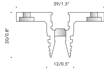
montantelettrico mb1 2000/3000mm 78.7"/118.1" scala · scale 1:1
