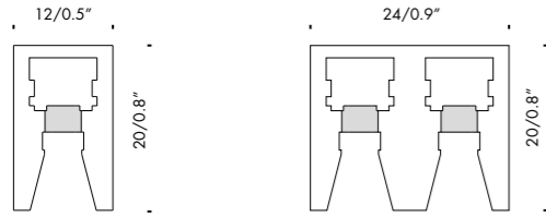
montantelettrico ma1 2000/3000mm 78.7"/118.1" scala · scale 1:1
