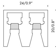
montantelettrico ma2 2000/3000mm 78.7"/118.1" scala · scale 1:1
