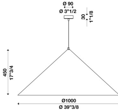
Technical drawing Size ref. image mm - inch
